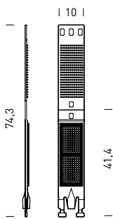
9. RA24---- MASSAGING STRIP for wall mounting, washer, 1/2" fitting.
