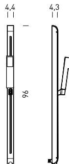
8. RA23---- SHOWER RAIL ON TRACK shower unit with riser track, anti-lime scale shower system, 960 mm in length, 1500 mm long flexible hose, chromed brass and steel finishes, built-in 1/2" wall fitting.
