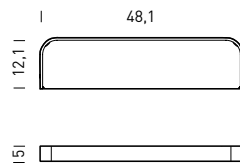
10. K040---- ACCESSORY SHELF 480 mm width, 120 mm width, chromed brass and steel finishes.
