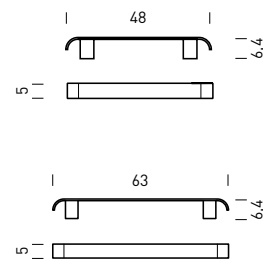
11. K041----, K042---- TOWEL RAIL, 630 or 480 mm length, chromed brass body.
